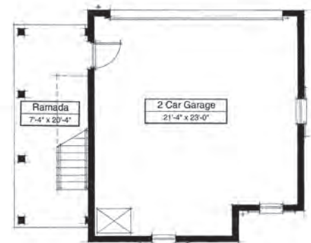
FIRST FLOOR PLAN 1/8"=1'-0"
